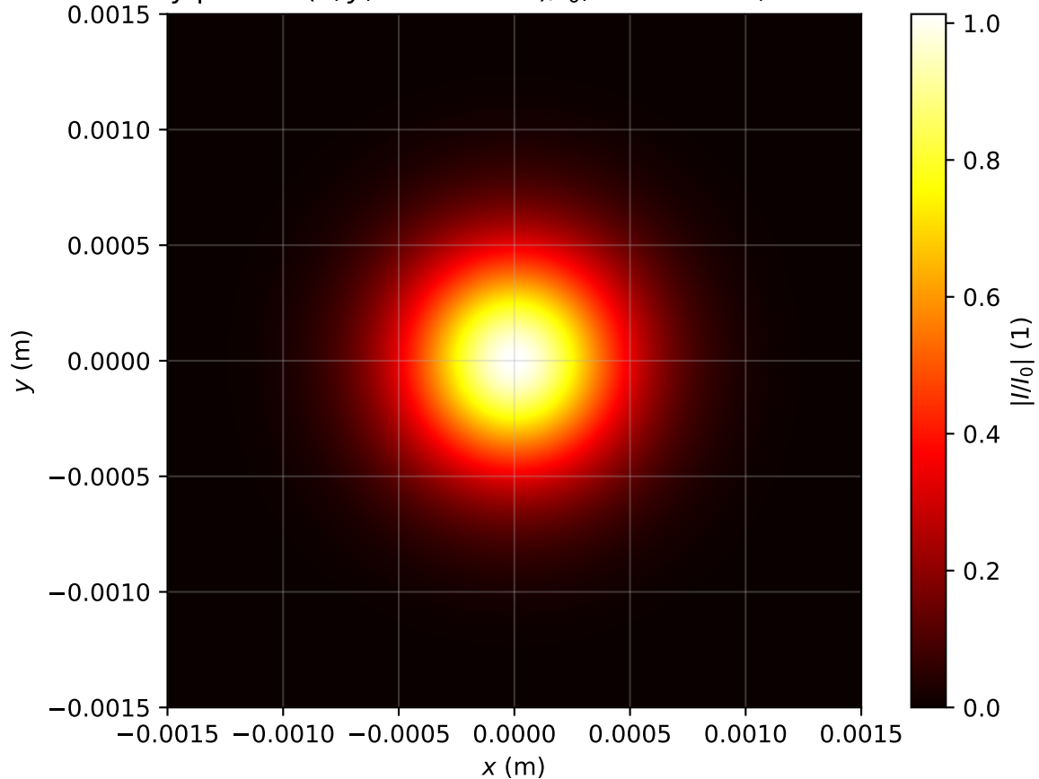
Intensity profile I(x, y, z = 0.796m)/I_0 , Pin=0.4Pcr, artificial time
